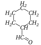
Cyclohexylmethanal
