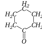
Cyclohexanone
