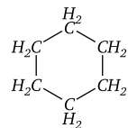
Cyclohexane
